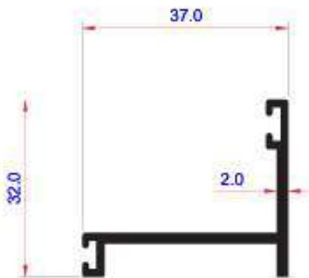
12402 0.415 kg/m
