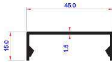
12401 0.337 kg/m
