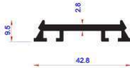
12400 0.448 kg/m
